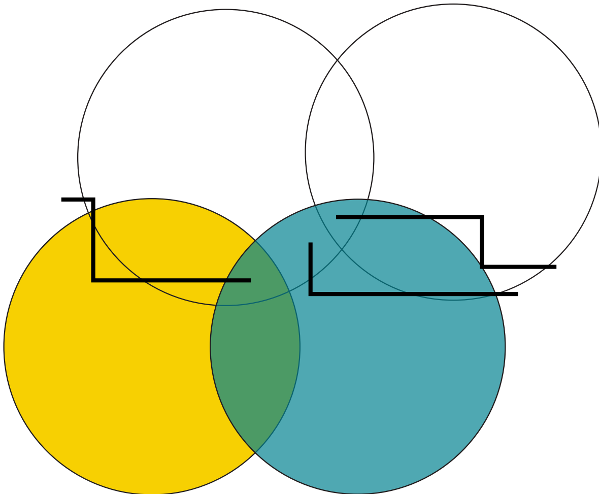
FIGURE 3: NETWORK HIESRARCHY
